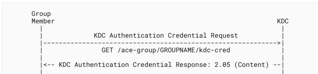
Figure 21: Message Flow of KDC Authentication Credential Request-Response to Obtain the Authentication Credential of the KDC
