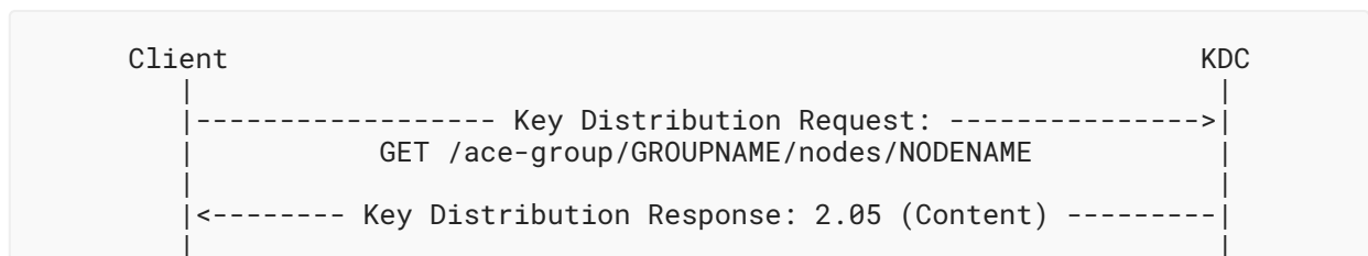
Figure 27: Message Flow of Key Distribution Request-Response
