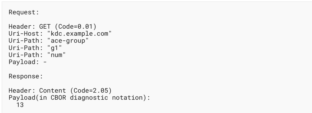
Figure 26: Example of Version Request-Response
