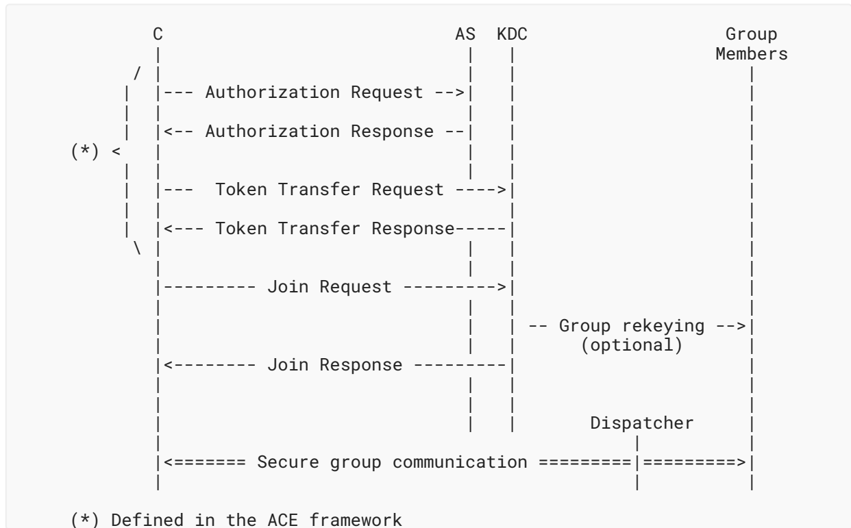
Figure 2: Message Flow upon a New Node's Joining
