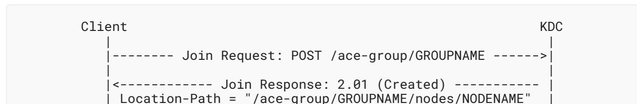
Figure 12: Message Flow of the Join Request-Response
