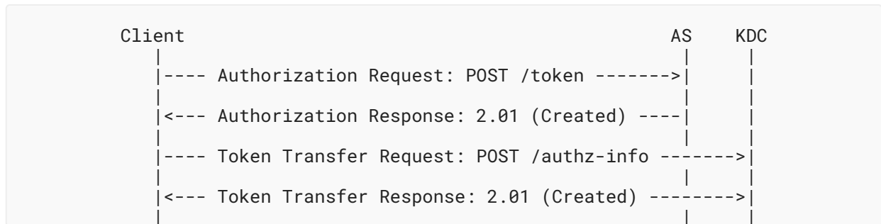
Figure 3: Message Flow of Join Authorization
