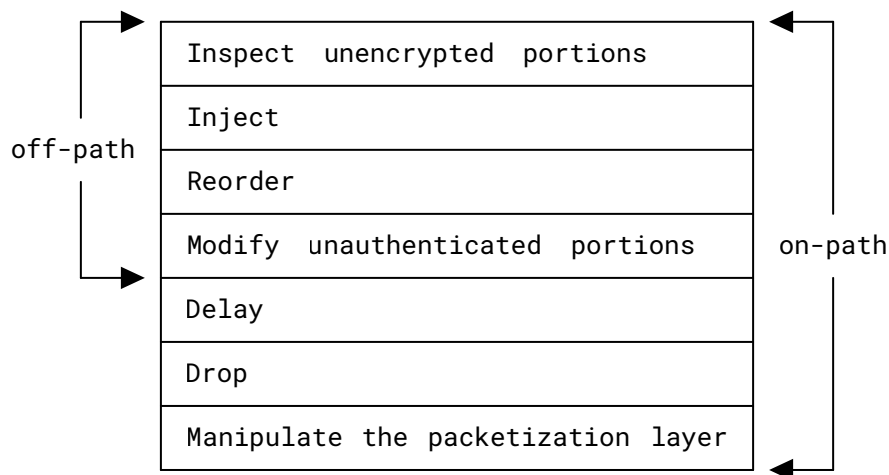
Figure 4: Attacker Capabilities
