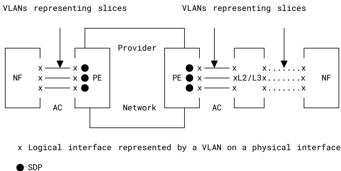
Figure 12: Example of 5G Network Slice with VLAN Handoff Providing End-to-End Connectivity
