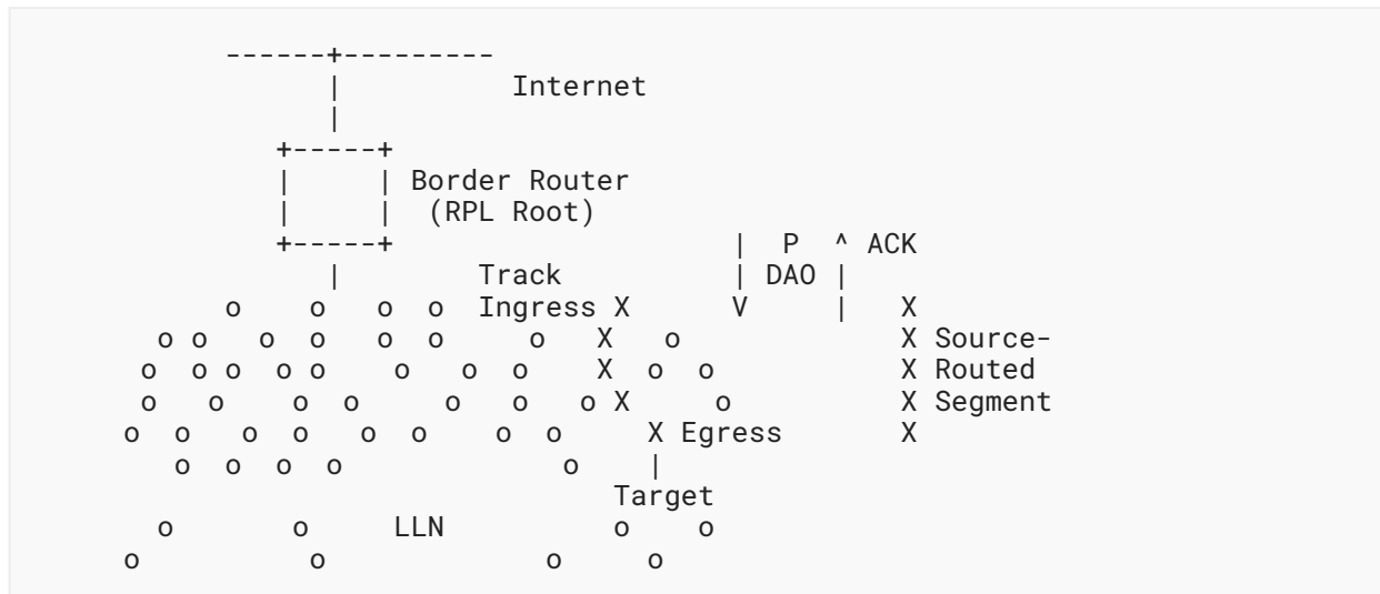
Figure 19: Projecting a Non-Storing Route
