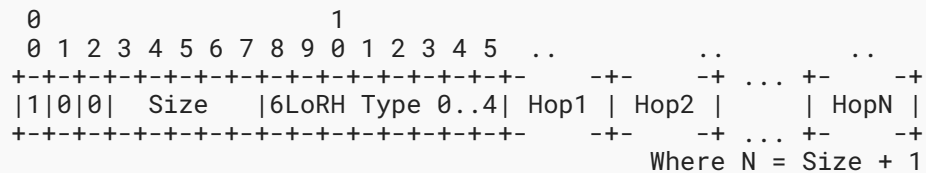
Figure 22: The SRH-6LoRH Header
