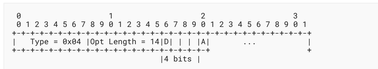
Figure 10: DODAG Configuration Option (Partial View)
