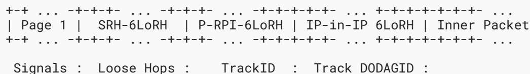
Figure 23: A Packet as Forwarded Along a Track
