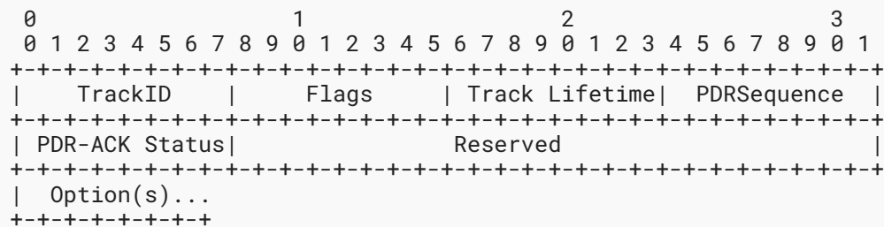
Figure 14: New PDR-ACK Control Message Format
