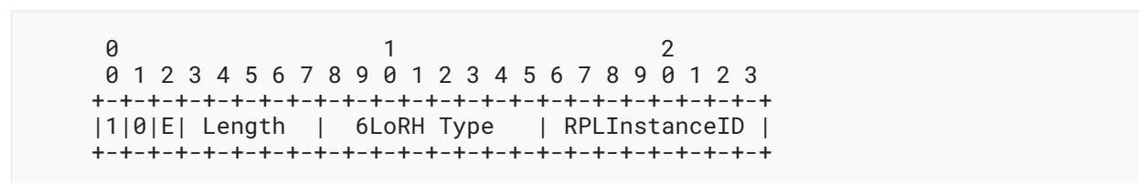
Figure 12: P-RPI-6LoRH Format
