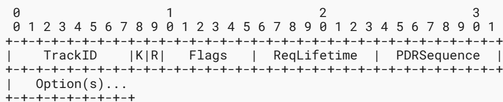
Figure 13: New P-DAO Request Format
