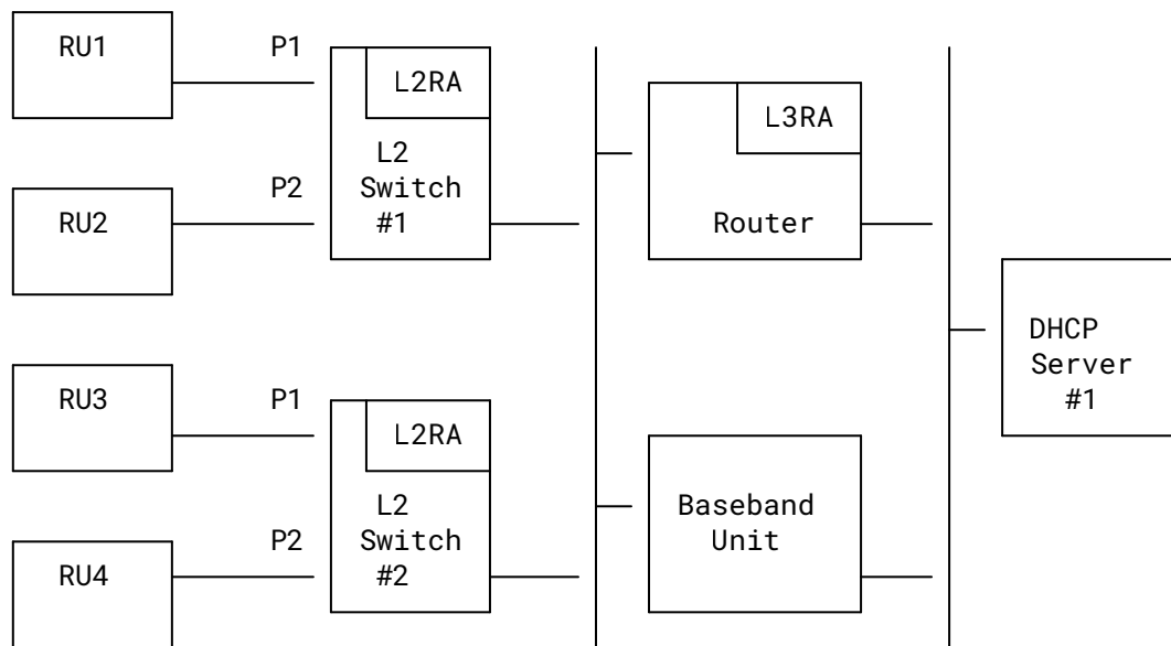
Figure 6: 3GPP RAN with Layer 2 Switched Fronthaul Example
