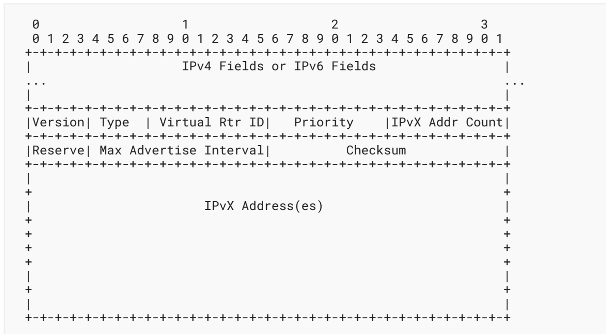
Figure 1: IPv4/IPv6 VRRP Advertisement Packet Format
