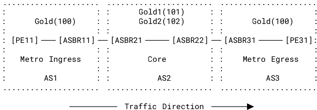
Figure 9: Transport Layer with Heterogenous Color Domains
