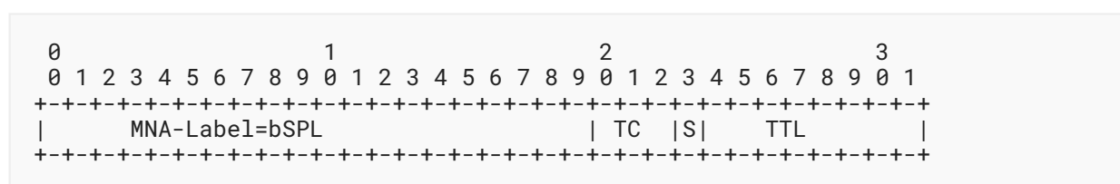
Figure 2: LSE Format A: The MNA Sub-Stack Indicator
