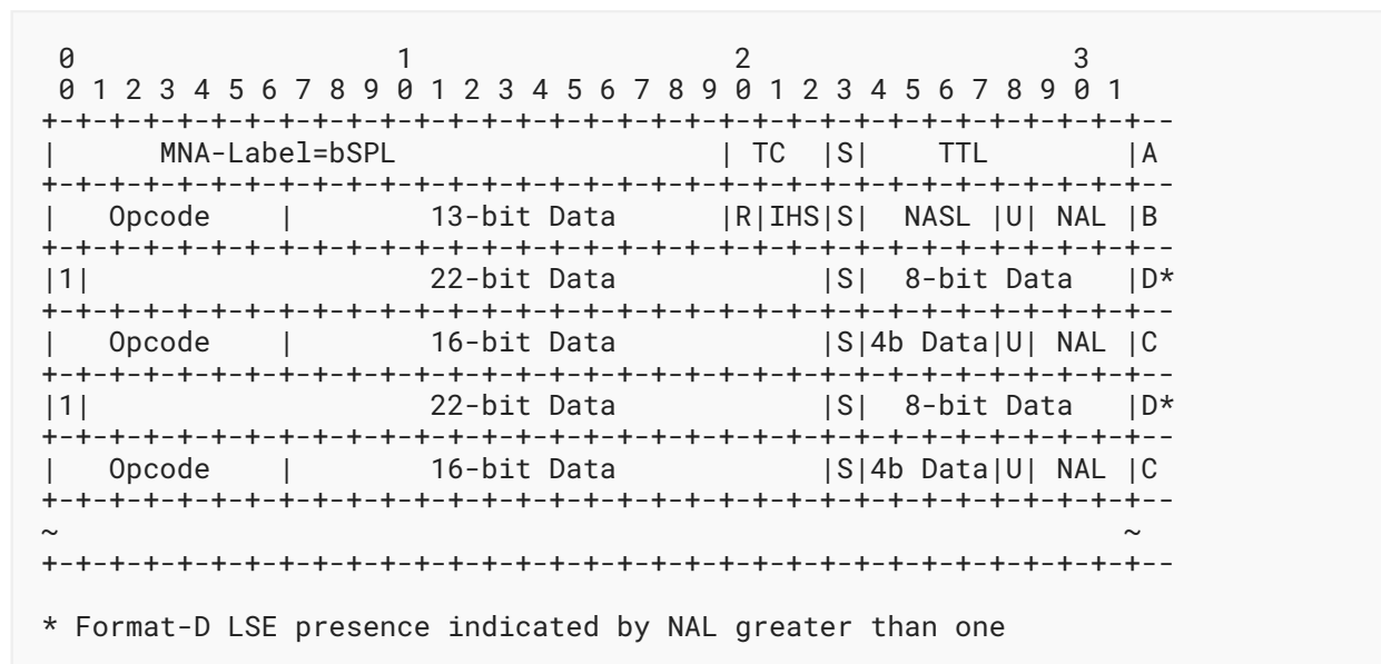
Figure 1: An MNA Sub-Stack Encoding Example
