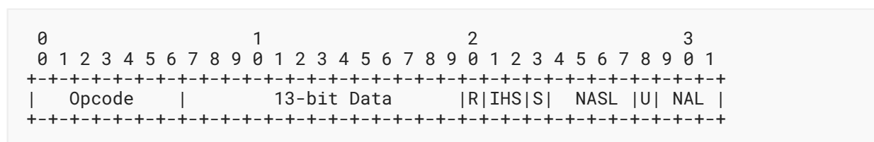
Figure 3: LSE Format B: The Initial Opcode
